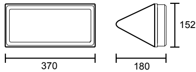
PF Decke / ceiling
