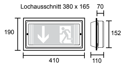
PF Einbau / recessed
